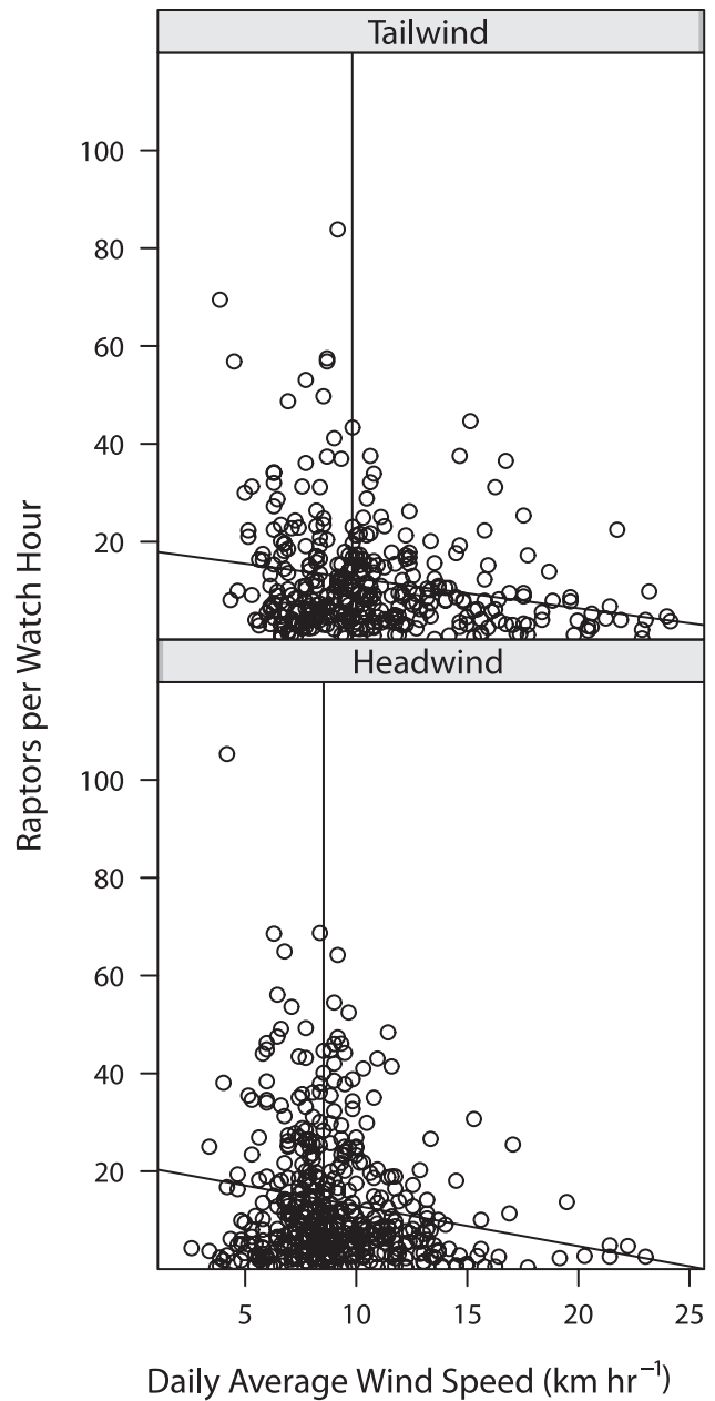
FIGURE 4. Overall counts of raptors (per watch hour) as compared to daily average wind speed ( \text{km hr}^{-1} ) for favorable tailwinds (upper) and unfavorable headwinds (lower). Vertical line, median; diagonal line, trend.
